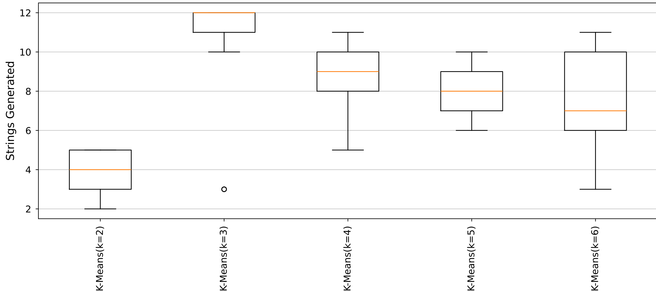
YARA Rules Strings Generated Distribution (Cluster23_Size6 dataset)
